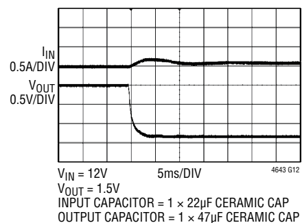
Short-Circuit with No Load Applied
