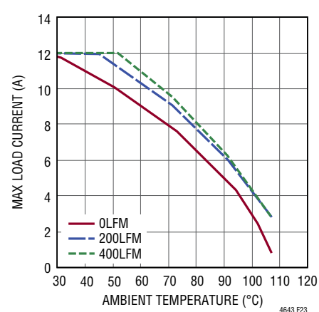
Figure 23. 12V IN to 3.3V OUT Derating Curve, 4-Channel Paralleled, No Heat Sink
