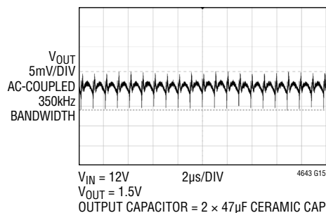
Output Ripple
