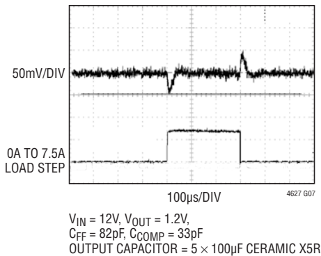
1.2V Transient Response
