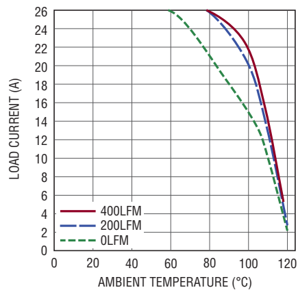
Figure 21. 5V to 2.5V Derating Curve, BGA Heat Sink
