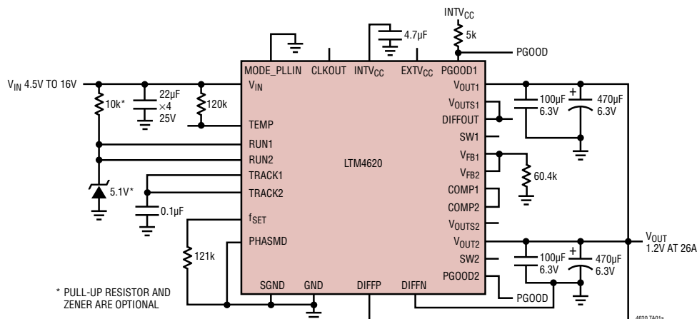
26A, 1.2V Output DC/DC \mu Module ® Regulator
