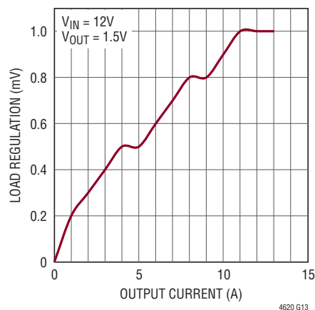
Load Regulation vs Current
