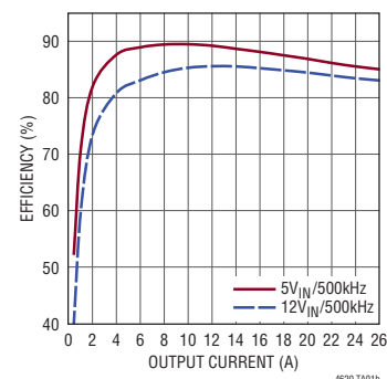
1.2V Efficiency vs I_{OUT}
