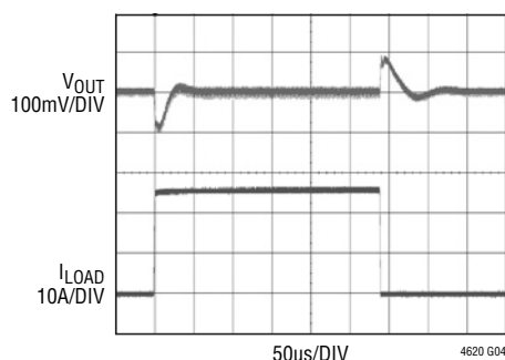
Dual Phase Single Output Load Transient Response
