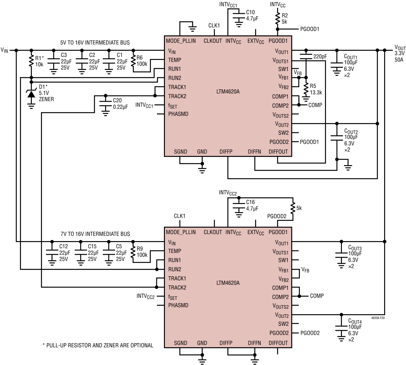
Figure 29. 4-Phase, 3.3V at 50A, 750kHz
