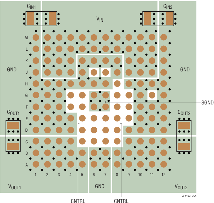
Figure 25. Recommended PCB Layout
