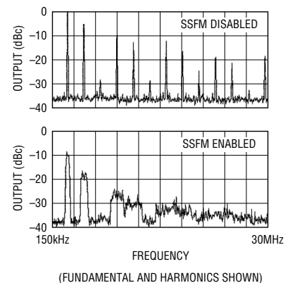
150kHz to 30MHz Output Frequency Spectrum (9kHz Res BW)
