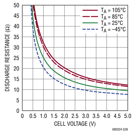
Internal Discharge Resistance vs Cell Voltage
