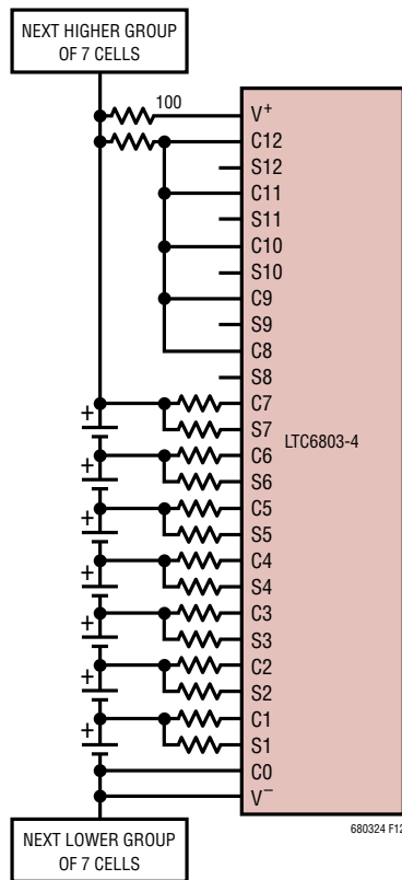
Figure 12. Monitoring 7 Cells with the LTC6803-4
