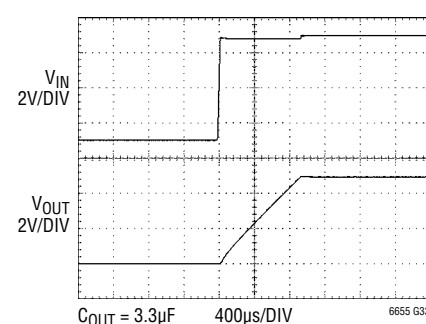
5V Start-Up Response with a 3.3μF Output Capacitor
