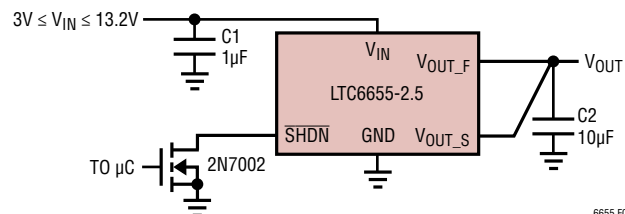
Figure 9. Open-Drain Shutdown Circuit
