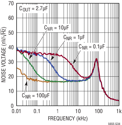
LTC6655LN-2.5 Output Voltage Noise Spectrum
