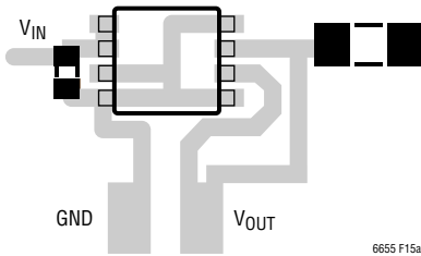
Figure 15a. Sample LTC6655 PCB Layout
