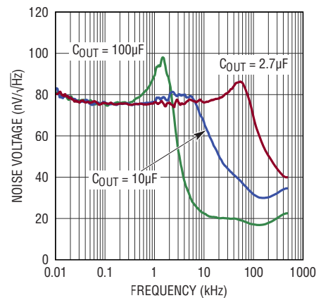
5V Output Voltage Noise Spectrum
