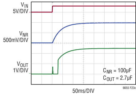
Figure 23c. C_{NR} = 100\mu\text{F}
