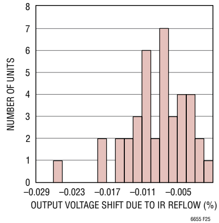
Figure 25. Output Voltage Shift Due to IR Reflow
