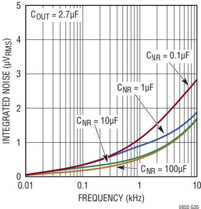
LTC6655LN-2.5 Output Integrated Noise
