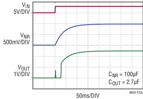
Figure 23c. C_{NR} = 100\mu\text{F}
