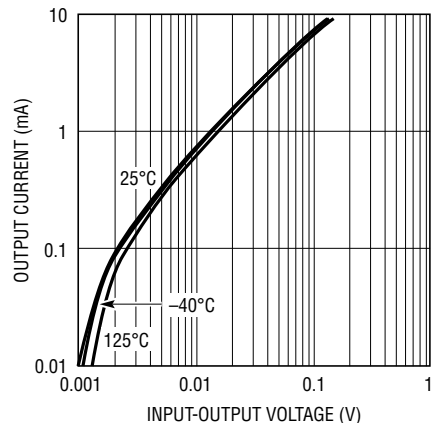
5V Minimum V IN to V OUT Differential (Sourcing)
