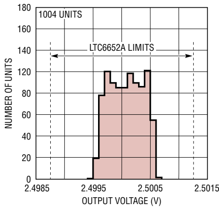
Typical V_{\text{OUT}} Distribution for LTC6652-2.5
