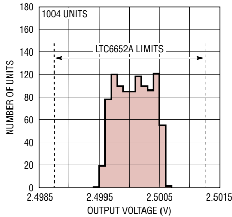
Typical V_{\text{OUT}} Distribution for LTC6652-2.5
