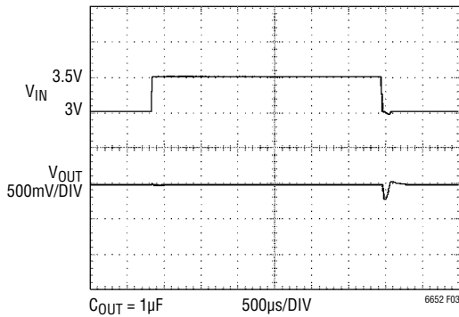
Figure 3. Transient Response with 1 \mu F Output Capacitor
