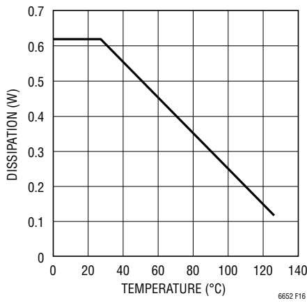
Figure 16. Maximum Recommended Dissipation for LTC6652
