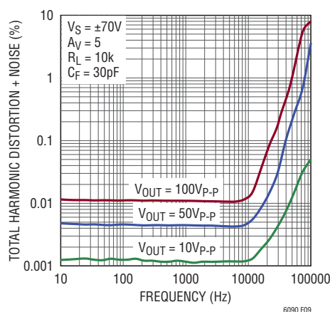
Figure 9. Distortion vs Frequency for Large Output Swings
