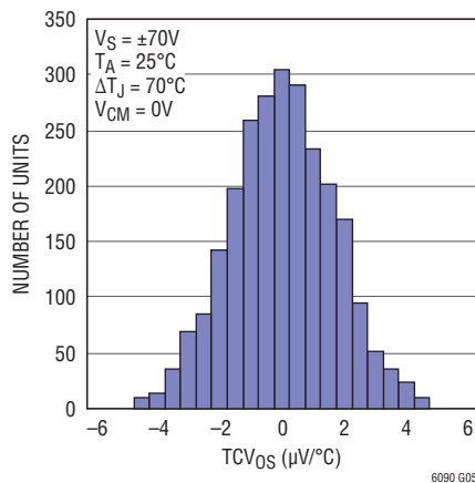
TCV_{OS} Distribution
