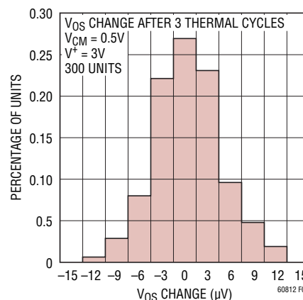
Figure 1. V_{OS} Thermal Hysteresis of LTC6081MS8
