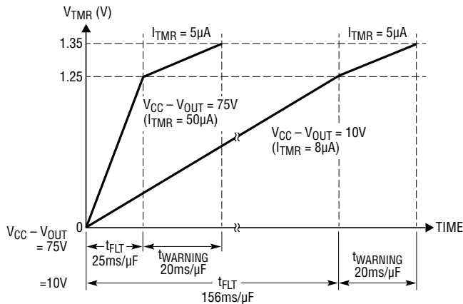
(a) Overvoltage Fault Timer Current
