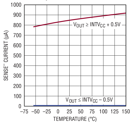
SENSE - Pin Input Bias Current vs Temperature
