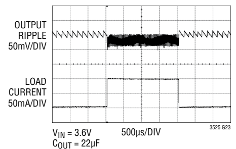
LTC3525-5 100mA Load Step Response
