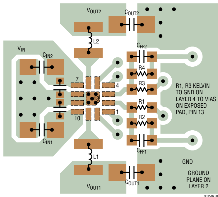
Figure 3. Recommended LTC3315A LQFN PCB Layout
