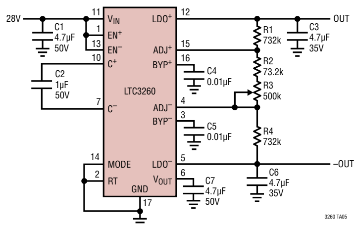
28V Dual Tracking Bipolar Supply with Outputs from \pm 5\text{V} to \pm 25\text{V}
