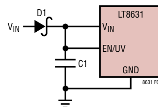
Figure 4. Reverse Input Voltage Protection
