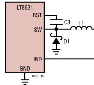
Figure 6. External Schottky Catch Diode
