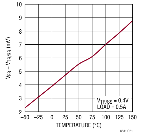
FB to TR/SS Offset Voltage
