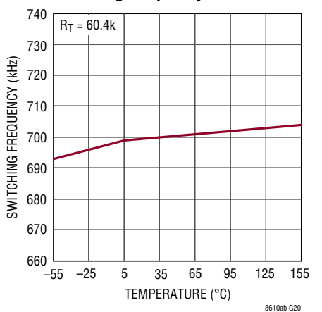
Switching Frequency
