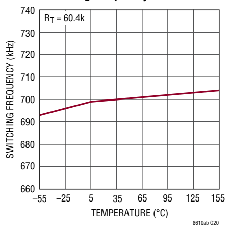
Switching Frequency
