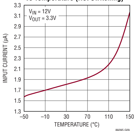
No-Load Supply Current vs Temperature (Not Switching)
