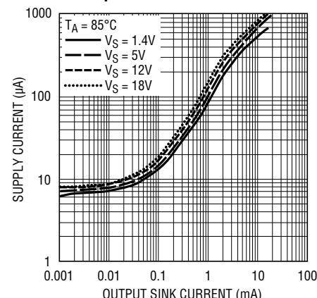
Supply Current vs Output Sink Current
