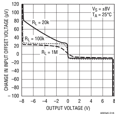
Open-Loop Gain
