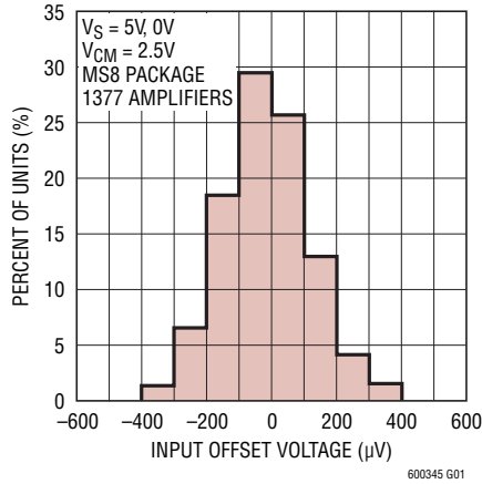
V_{OS} Distribution
