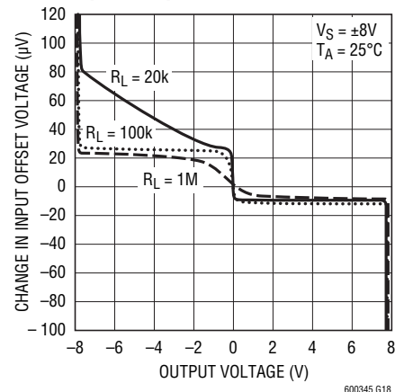
Open-Loop Gain
