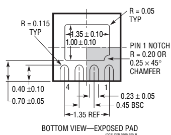
BOTTOM VIEW—EXPOSED PAD (DCA) DFN 0300 REV B
