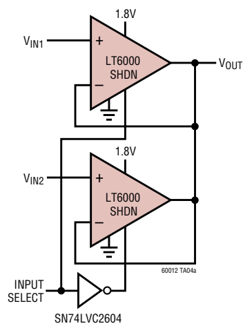
MUX Amplifier
