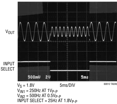
MUX Amplifier Waveforms
