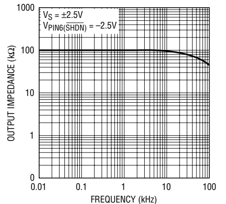
Disabled Output Impedance vs Frequency (LT6000/LT6001DD)
