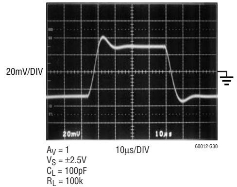
Small-Signal Response
