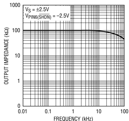
Disabled Output Impedance vs Frequency (LT6000/LT6001DD)
