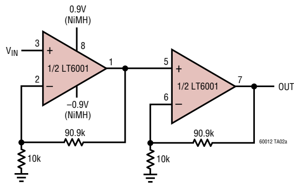
Gain of 100 Amplifier (400kHz GBW on 30μA Supply)
