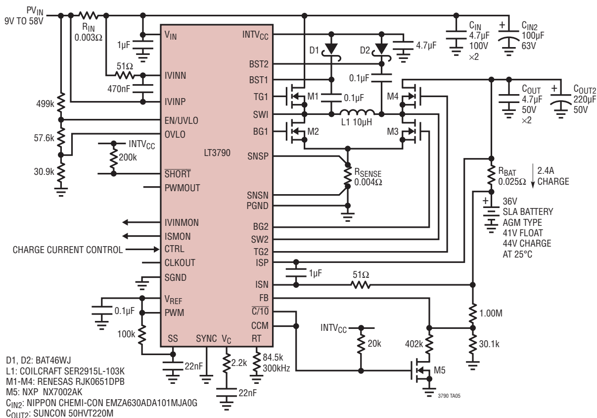
2.4A Buck-Boost 36V SLA Battery Charger
