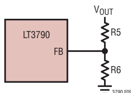
Figure 9. Resistor Connection for Constant Output Voltage Regulation
