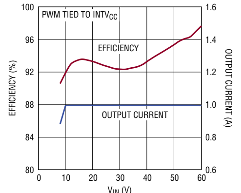
Boost Efficiency and Output Current vs V_{IN}
