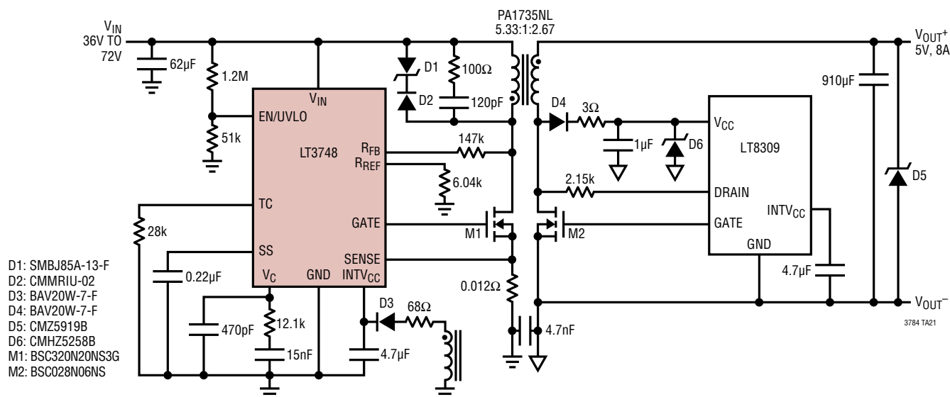
Figure 21. 5V, 8A Isolated Supply with Synchronous Secondary-Side Rectification Using LT8309
