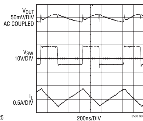
Switching Waveforms for Figure 14 Circuit
