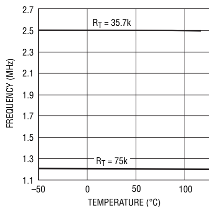
Oscillator Frequency
