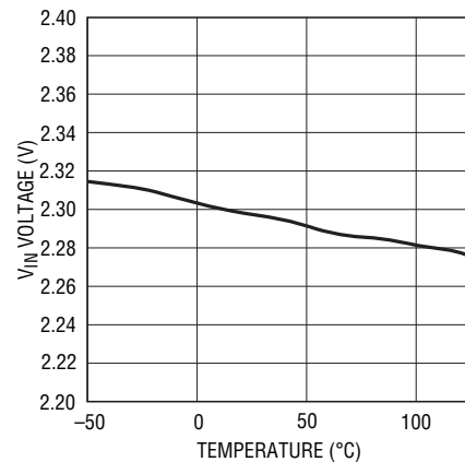
Internal UVLO
