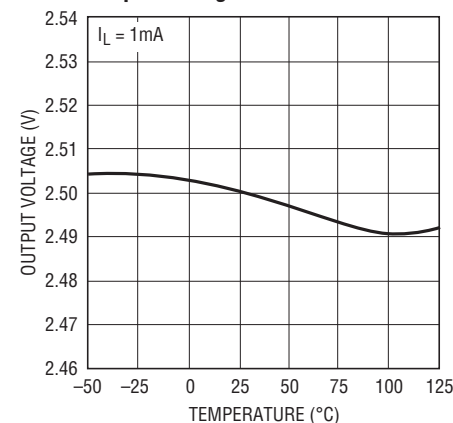
LT1761-2.5 Output Voltage
