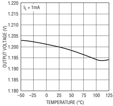
LT1761-1.2 Output Voltage
