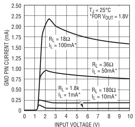
LT1761-1.8 GND Pin Current
