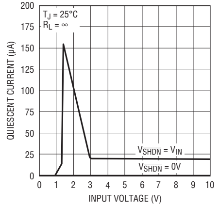
LT1761-3 Quiescent Current
