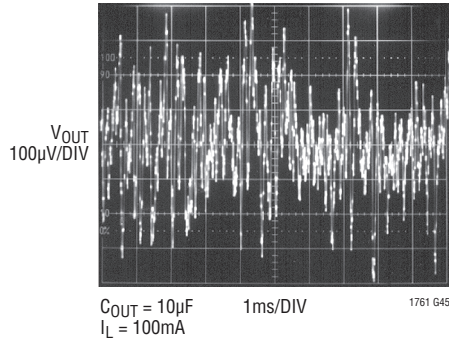
LT1761-5 10Hz to 100kHz Output Noise C_{BYP} = 0\text{pF}
