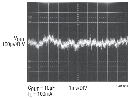
LT1761-5 10Hz to 100kHz Output Noise C_{BYP} = 1000\text{pF}
