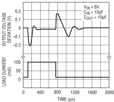
LT1761-5 Transient Response C_{BYP} = 0\text{pF}
