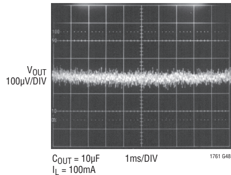
LT1761-5 10Hz to 100kHz Output Noise C_{BYP} = 0.01\mu\text{F}
