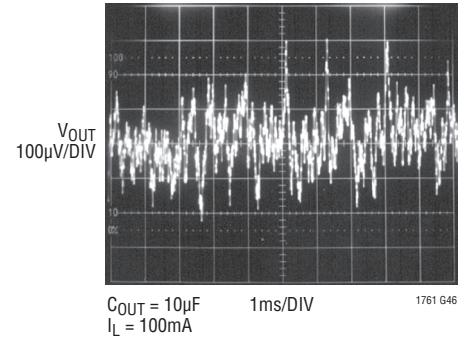
LT1761-5 10Hz to 100kHz Output Noise C_{BYP} = 100\text{pF}
