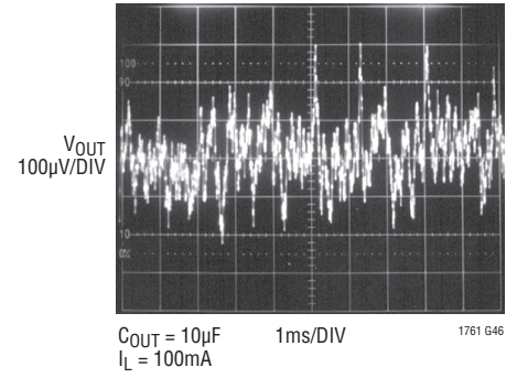
LT1761-5 10Hz to 100kHz Output Noise C_{BYP} = 100\mu F
