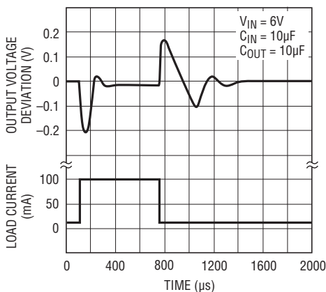
LT1761-5 Transient Response C_{BYP} = 0\mu F
