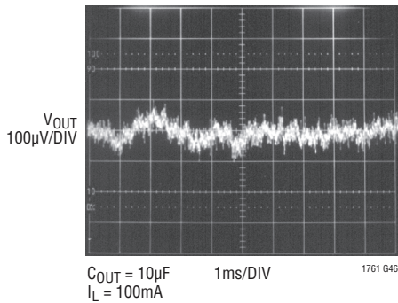
LT1761-5 10Hz to 100kHz Output Noise C_{BYP} = 1000\mu F
