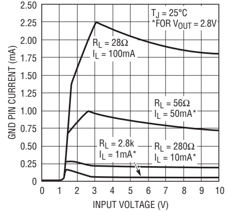
LT1761-2.8 GND Pin Current
