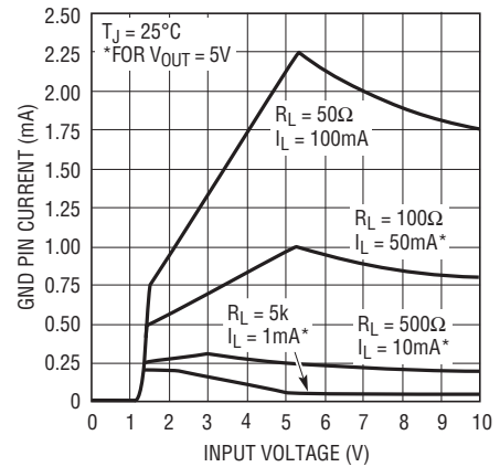
LT1761-5 GND Pin Current
