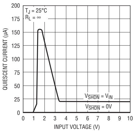
LT1761-3.3 Quiescent Current
