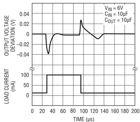
LT1761-5 Transient Response C_{BYP} = 0.01\mu F
