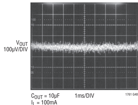
LT1761-5 10Hz to 100kHz Output Noise C_{BYP} = 0.01\mu F
