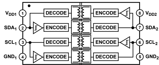
Figure 1. ADuM1250
