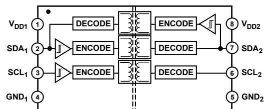
Figure 2. ADuM1251
