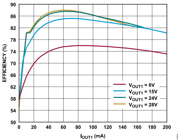
Figure 7. Overall Efficiency at Various V_{OUT1} Output Voltages, T_A = 25^\circ\text{C} , V_{INP} = 24\text{ V} , V_{OUT2} = 5.0\text{ V} , I_{OUT2} = 6\text{ mA} , V_{OUT3} = -15\text{ V} , I_{OUT3} = -4\text{ mA}
