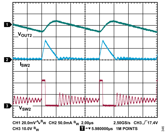
Figure 46. Buck Regulator Discontinuous Conduction Mode Operation Showing I_{SW2} , Switch Node Voltage, and Output Ripple, T_A = 25^\circ\text{C} , V_{OUT1} = 24\text{ V} , V_{OUT2} = 5\text{ V} , I_{OUT2} = 11\text{ mA}
