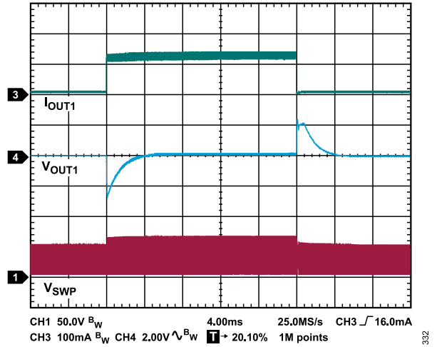
Figure 32. Flyback Regulator Load Transient Response, V_{VINP} = 24\text{ V} , V_{OUT1} = 24\text{ V} , I_{OUT1} = 4\text{ mA} to 120\text{ mA} Step, T_A = 25^\circ\text{C}
