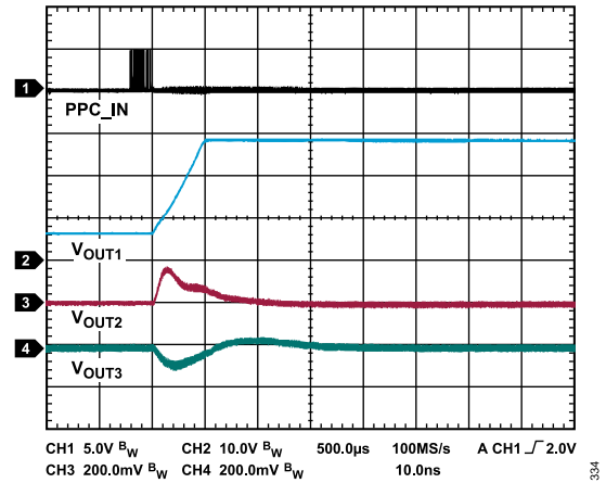
Figure 34. PPC Full Output Range Step, from V_{OUT1} = 6\text{ V} to 28\text{ V} , V_{VINP} = 24\text{ V} , V_{OUT1} Load = 1\text{ k}\Omega , V_{OUT2} = 5.0\text{ V} , I_{OUT2} = 6\text{ mA} , V_{OUT3} = -15\text{ V} , I_{OUT3} = -4\text{ mA} , T_A = 25^\circ\text{C}
