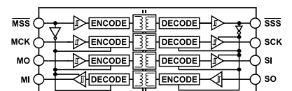
Figure 79. iCoupler Gating
