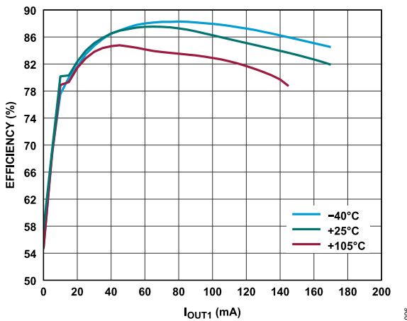
Figure 6. Overall Efficiency Across Temperature, V_{INP} = 24\text{ V} , V_{OUT1} = 24\text{ V} , V_{OUT2} = 5.0\text{ V} , I_{OUT2} = 6\text{ mA} , V_{OUT3} = -15\text{ V} , I_{OUT3} = -4\text{ mA}
