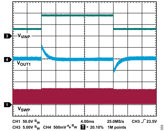
Figure 33. Flyback Regulator Line Transient Response, V_{VINP} = 18\text{ V} to 24\text{ V} , V_{OUT1} = 24\text{ V} , I_{OUT1} = 100\text{ mA} , T_A = 25^\circ\text{C}
